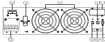
b. 0.9PF 2KVA RT arka paneli
